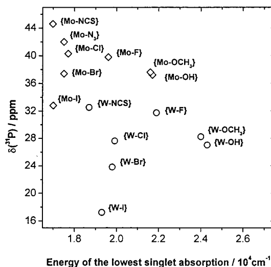
Figure 3. Plot showing the correspondence between the energy of the first band maximum in the absorption spectrum and the chemical shift of the phosphorus nuclei. The complexes have been abbreviated by the metal and the trans -to-oxygen ligand.
