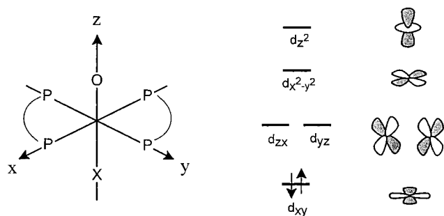
Figure 1. Coordinate system employed for the trans -[M(O)(X)(dppe) _2 ] ^{+/0} complexes. The orbital splitting pattern together with the orbital population in the resulting low-spin d^2 system are depicted on the right.
