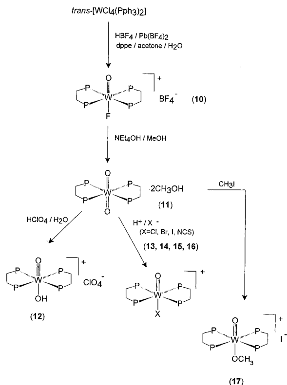
Scheme 2. Schematic Representation of the Synthetic Routes to the Tungsten Complexes and Labeling Scheme for These
