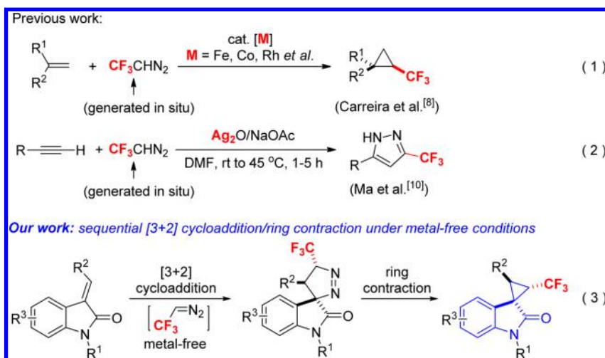
Scheme 2. Design of the [3 + 2] Cycloaddition/Ring Contraction Sequence for the Synthesis of CF 3 -Containing 3,3'-Cyclopropyl Spirooxindoles
