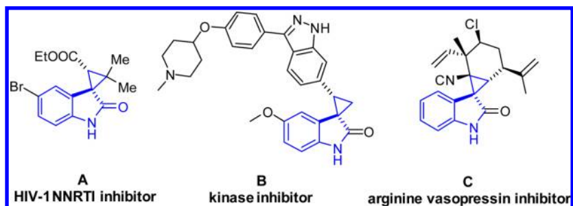
Scheme 1. Representative Therapeutic Agents Containing 3,3'-Cyclopropyl Spirooxindole Scaffolds
