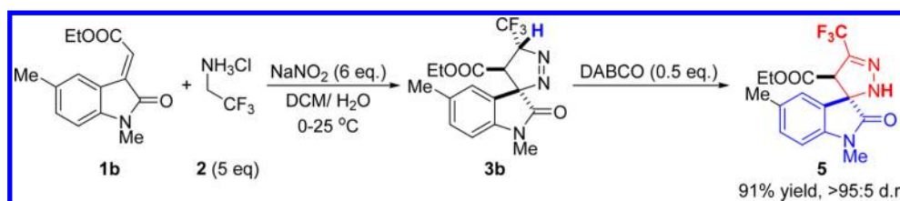
Scheme 4. Sequential [3 + 2] Cycloaddition/1,3-H Shift Reaction for the Synthesis of CF 3 -Containing Spiropyrzoline Oxindole 5
