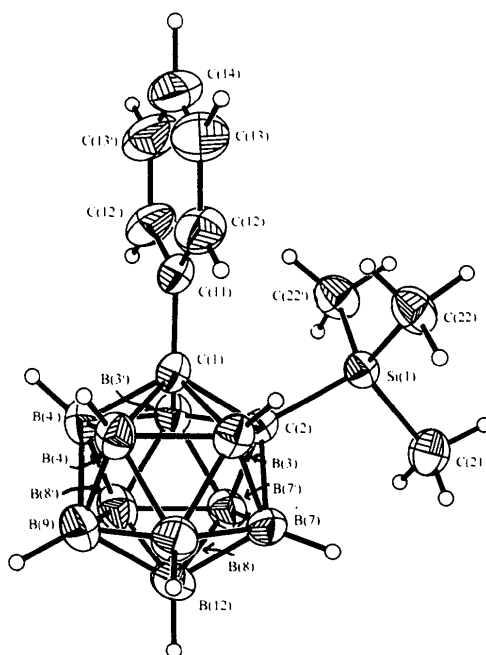
Fig. 1. A perspective view of 1-Ph-2-Me 3 Si-1,2- closo - C_2B_{10}H_{10} . Displacement ellipsoids are shown at the 50% probability level for non-H atoms and H atoms are represented by spheres with arbitrary radii of 0.1 Å. [Symmetry code: (i) x, \frac{1}{2} - y, z .]
