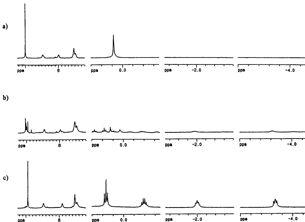
Fig. 4. Partial ^1\text{H} -NMR (500 MHz, \text{C}_7\text{D}_8 ) spectra of stepwise reaction of (\text{TPP})\text{Hf}(\text{OAc})_2 with \text{nBuLi} . (a) (\text{TPP})\text{Hf}(\text{OAc})_2 ; (b) after addition of 2 equiv. of \text{nBuLi} to (a); (c) after addition of 4 equiv. of \text{nBuLi} to (a).
