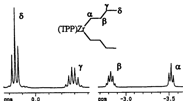
Fig. 3. Partial ^1\text{H} -NMR (300 MHz, \text{C}_7\text{D}_8 ) spectrum of (\text{TPP})\text{Zr}(\text{nBu})_2 formed from the addition of 2 equiv. of \text{nBuLi} to (\text{TPP})\text{ZrCl}_2 .
