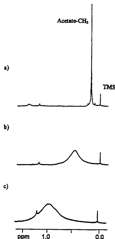
Fig. 2. 1 H-NMR (300 MHz, CDCl 3 ) spectra, acetate region only. (a) (TPP)Zr(OAc) 2 ; (b) after addition of 0.4 equiv. of HOAc to (a); (c) after addition of 1.2 equiv. of HOAc to (a).
