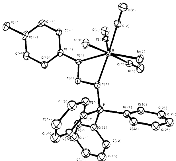
Figure 1. Drawing of a molecule of \text{WBr}_2(\text{CO})_3(p\text{-CH}_3\text{C}_6\text{H}_4\text{N}_3\text{PPh}_3) . The hydrogen atoms have been omitted. Vibrational ellipsoids are drawn at the 50% probability level.
