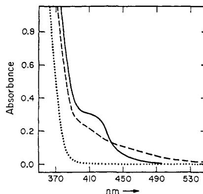
Figure 1. Spectral changes in the uv-visible region due to photochemical formation of [W(CO) 6 ( cis -stilbene)] (—) and [W(CO) 6 ( trans -stilbene)] (---) from 366-nm irradiation of W(CO) 6 (···).
