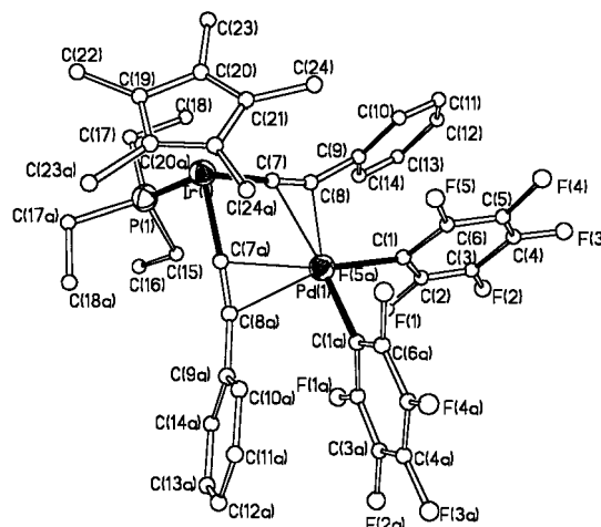
Figure 6. View of the molecular structure of complex 8a , showing the atom-numbering scheme. Hydrogen atoms have been omitted for clarity.
