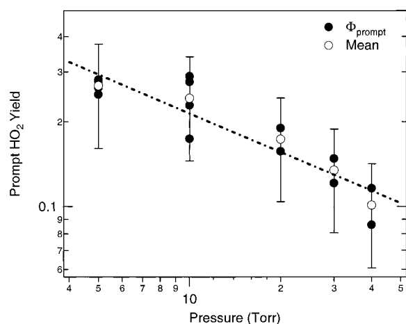
Figure 9. The pressure dependence of the prompt yield of \text{HO}_2 from the reaction of c\text{-C}_5\text{H}_9 + \text{O}_2 at 638 K and at a constant \text{O}_2 density of 6.6 \times 10^{16} \text{ molecule cm}^{-3} . The mean values are shown as the open circles \circ and the individual determinations as the filled circles \bullet . The dash-dotted line is the best fit to a P^{-n} dependence, shown for reference.
