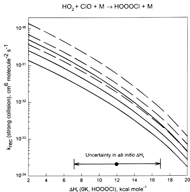
Figure 8. Rate constants for the reaction HO 2 + ClO + M → HOOOCl + M vs \Delta H_f^\circ(0\text{K}) for HOOOCl at 300 K (solid lines) and 200 K (dashed lines). At each temperature the uncertainty band associated with a \pm 10\% uncertainty in the HOOOCl vibrational frequencies is indicated.
