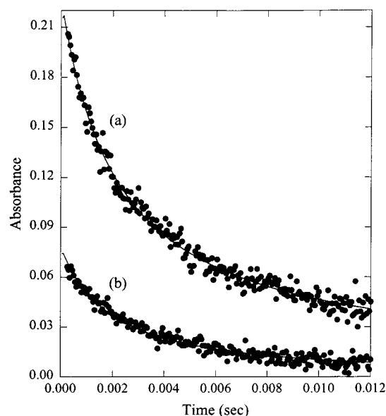
Figure 3. Example of time-resolved absorption signals for the F 2 -H 2 -O 2 -Cl 2 O system: (a) 210 nm absorption channel (HO 2 ); (b) differential absorption signal from 275.2 and 276.4 nm channels (ClO). The solid lines are fits obtained using FACSIMILE as discussed in the text.
