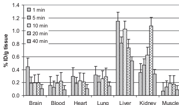
Figure 5. Biodistribution study of [ 11 C] 3 .
