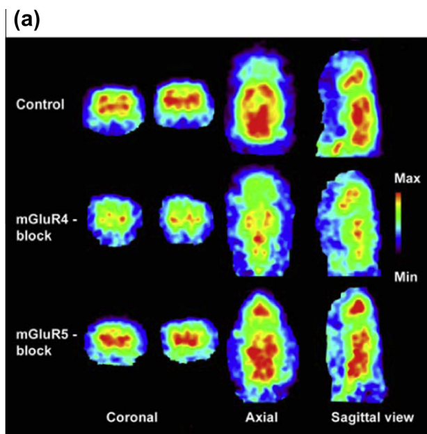
Figure 3. PET studies of specificity and selectivity of [ 11 C] 3 . (a) Comparison of [ 11 C] 3 distribution in rat brain at the time interval 2–15 min in a control study, after blocking of mGlu 4 with 4.HCl (10 mg/kg ip 30 min before [ 11 C] 3 injection) and after blocking of mGlu 5 with MTEP (5 mg/kg iv 2 min before [ 11 C] 3 ). Coronal images are at the striatal and hippocampal level while axial and sagittal views at the midstriatal level. (b) The uptake of [ 11 C] 3 was reduced by 23–28% in all brain areas with 4.HCl while MTEP induced blocking was minor.
