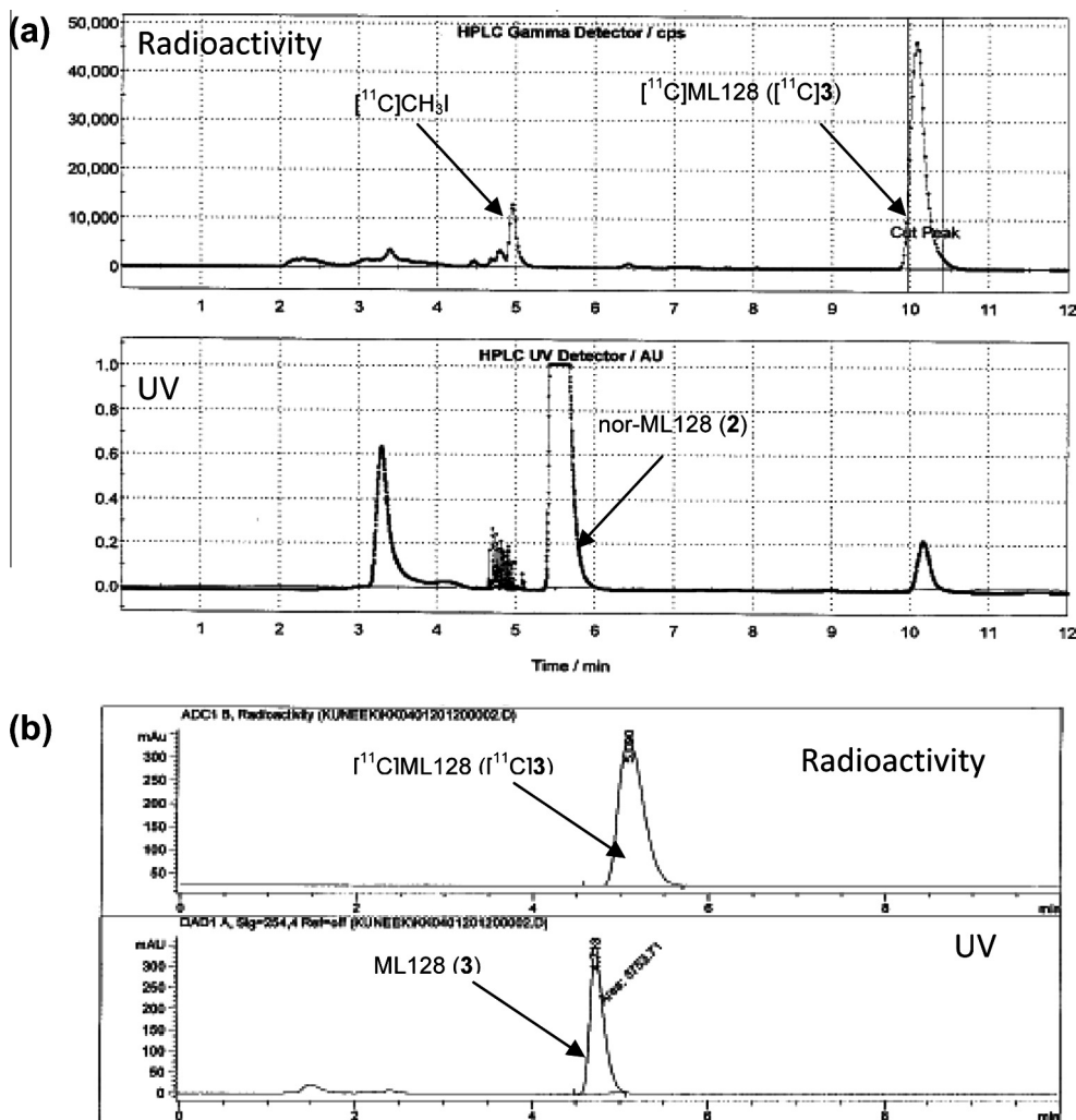
Figure 1. (a) UV and radioactivity traces of semi-preparative HPLC; (b) The analytical HPLC chromatogram for co-injection of [ 11 C] 3 with the cold reference 3 .
