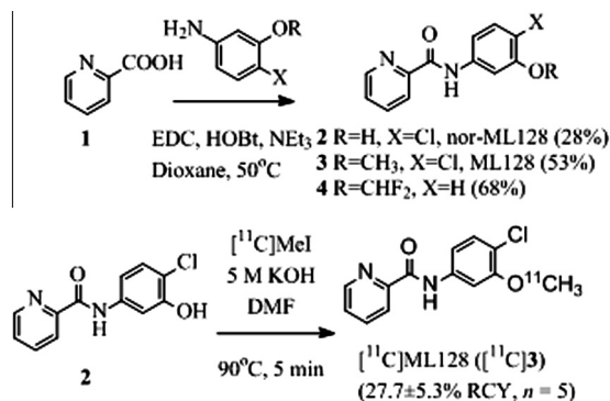
Scheme 1. Syntheses of reference ML128 ( 3 ), [ 11 C]ML128 ([ 11 C] 3 ), its precursor ( 2 ), and blocking agent ( 4 ).
