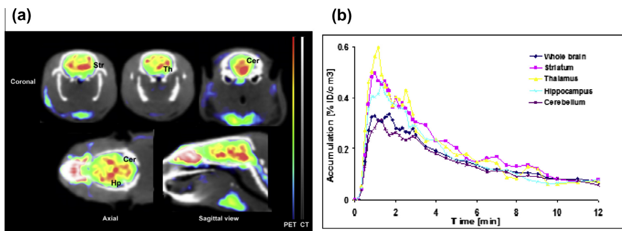
Figure 2. Pharmacokinetics of [ 11 C] 3 . (a) Representative cumulative PET/CT images of rat brain at the time interval 2–15 min after administration of [ 11 C] 3 (24.1 MBq iv). Slice thickness is 0.625 mm. Str = striatum, Hp = hippocampus, Th = thalamus and Cer = cerebellum. (b) TACs show fast uptake (peak activity between 1 and 3 min) followed by fast washout throughout the brain.
