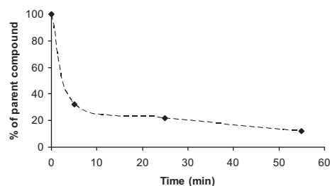
Figure 4. Metabolite corrected blood curve after [ 11 C] 3 injection.
