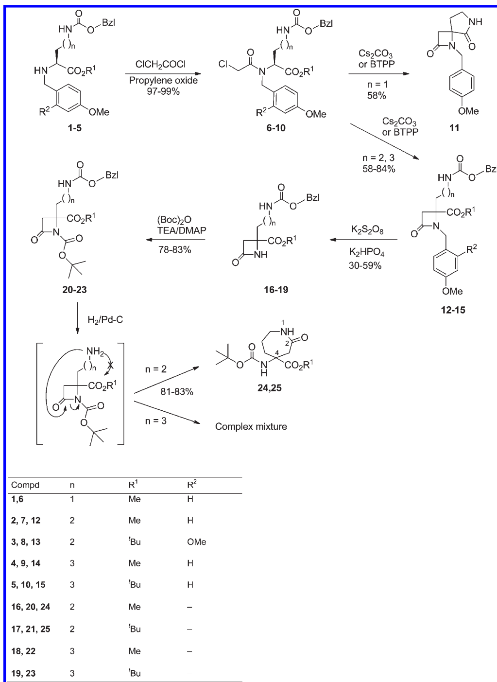
Scheme 1. Exploratory Attempts on the Formation of Heterocyclic Quaternary Amino Acids from \beta -Lactams
