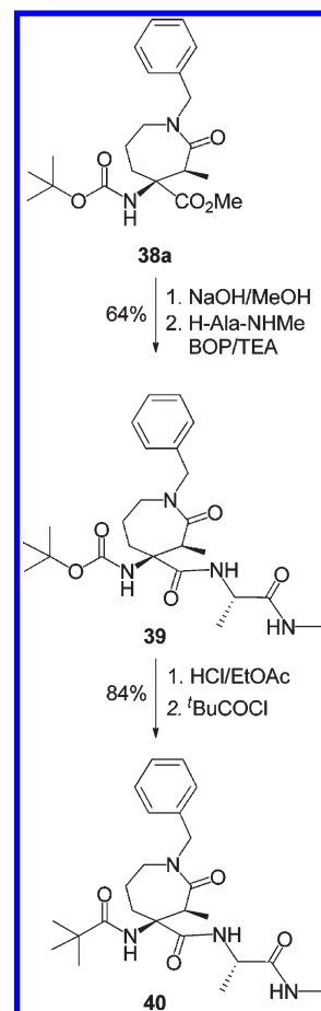
Scheme 3. Synthesis of 2-Oxoazepane-Containing Dipeptide Models
