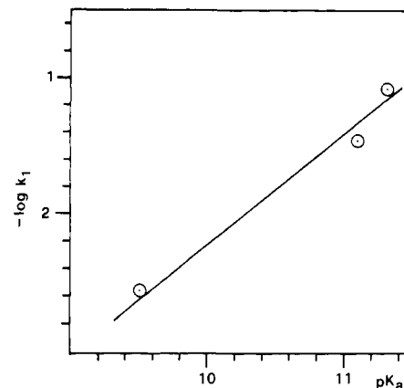
Figure 1. Effect of the basicity ( pK_a ) on the nucleophilic reactivity ( \log k_1 ) of the amine.
