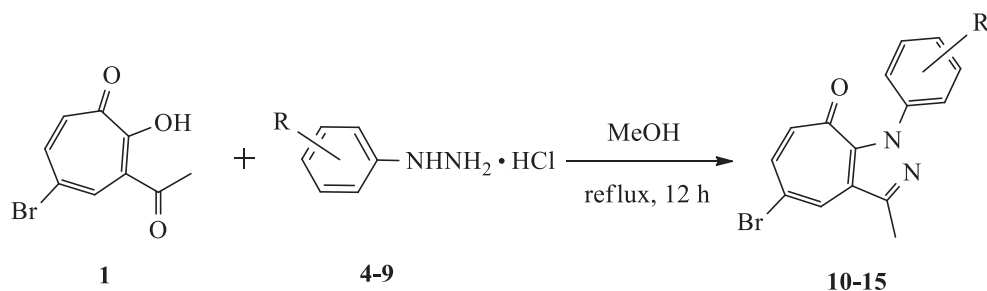
Scheme 2. Synthesis of 1-aryl-5-bromo-3-methyltropono[ c ]pyrazoles ( 10–15 ).
