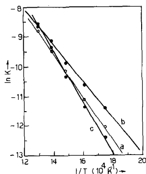
Fig. 3. Arrhenius plots for the isothermal decomposition of magnesium perchlorate: curve a, pure; curve b, mixed with 10 wt.% \text{CuV}_2\text{O}_6 catalyst; curve c, mixed with 10 wt.% \text{MgV}_2\text{O}_6 catalyst.
