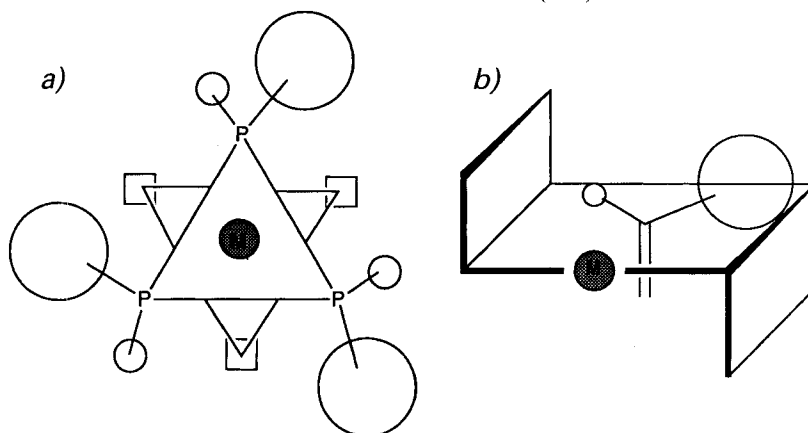
Fig. 1. a) The C_3 model in octahedral geometry, b) the C_2 model in square-planar geometry
