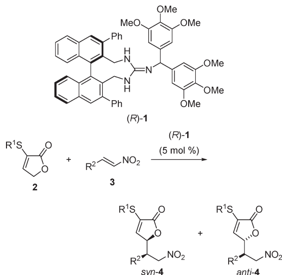
Scheme 1. Direct Vinylogous Michael Addition of \alpha -Thio Substituted Furanones 2 to Conjugate Nitroalkenes 3 Catalyzed by Axially Chiral Guanidine Base 1
