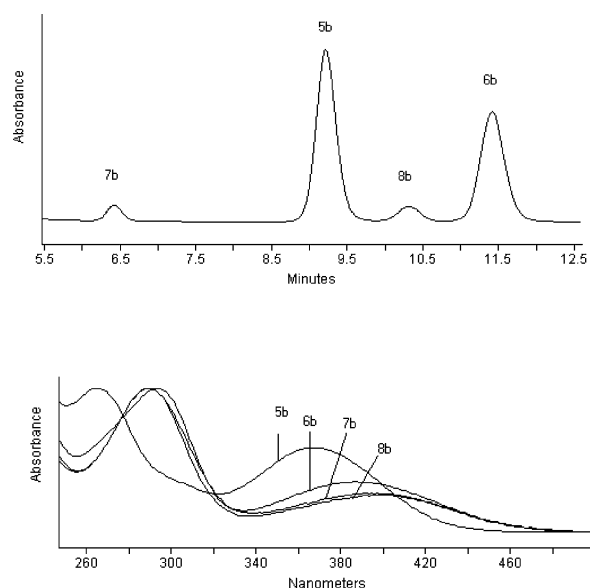
Fig. 3 (a) HPLC elution profile of crude mixture obtained from the reduction of salt 3b . The eluate was monitored at 275 and 380 nm. Retention times ( t_R ) start from injection point. (b) UV spectra were recorded on the top of the corresponding chromatographic peaks and are normalized with respect to their own \lambda_{\text{max}} .
