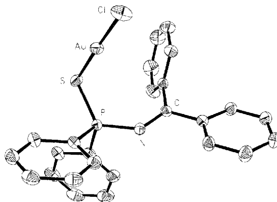
Figure 2. Molecular structure of 1aSAuCl (ORTEP, 50% probability ellipsoids, phenyl hydrogen atoms are omitted) [a]
