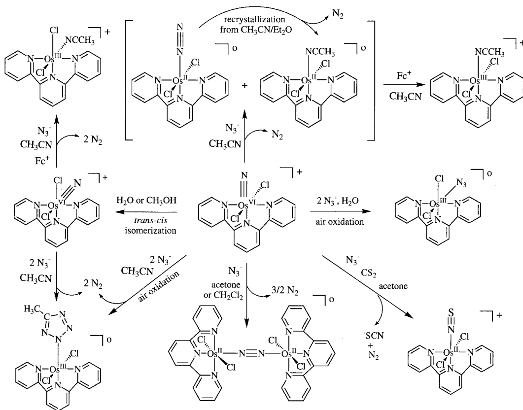
Figure 4. Reactivity between \text{trans-}[\text{Os}^{\text{VI}}(\text{tpy})(\text{Cl})_2(\text{N})]^+ ( 1 ) and \text{N}_3^- .
