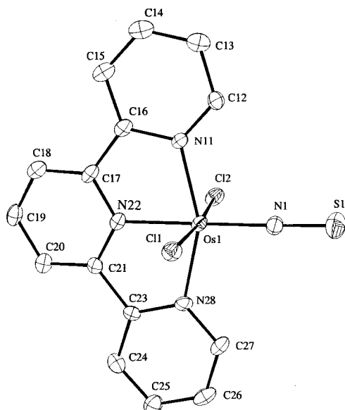
Figure 3. ORTEP diagram (30% probability ellipsoids) for the cation \text{trans-}[\text{Os}^{\text{II}}(\text{tpy})(\text{Cl})_2(\text{NS})]^+ in 14 .
