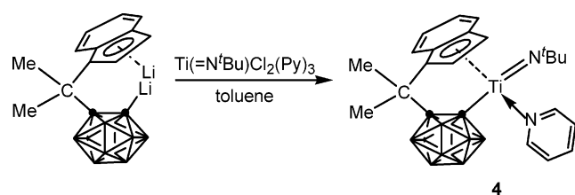
Figure 1. Molecular structure of [\eta^5:\sigma\text{-Me}_2\text{C}(\text{C}_5\text{H}_4)\text{-(C}_2\text{B}_{10}\text{H}_{10})]\text{Ti(=NC}_6\text{H}_3\text{Pr}_2^i\text{-2,6)(Py)} ( 3 ).
