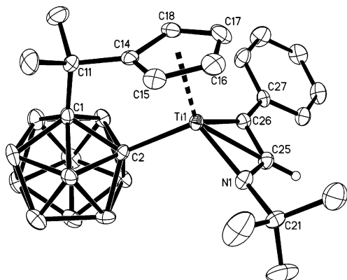
Figure 4. Molecular structure of [\eta^5\text{-}\sigma\text{-Me}_2\text{C}(\text{C}_5\text{H}_4)\text{-(C}_2\text{B}_{10}\text{H}_{10})]\text{Ti}(\eta^3\text{-N}^t\text{BuCH=CPh}) ( 6 ).
