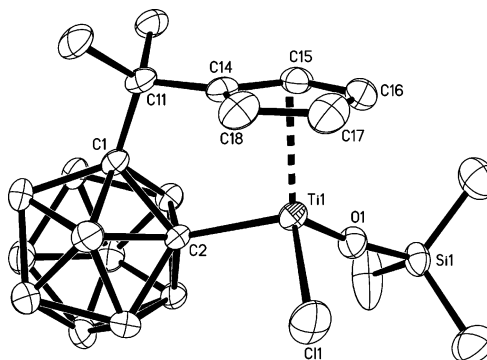
Figure 3. Molecular structure of [\eta^5:\sigma\text{-Me}_2\text{C}(\text{C}_5\text{H}_4)\text{-(C}_2\text{B}_{10}\text{H}_{10})]\text{Ti(OSiMe}_3\text{)Cl} ( 5 ).
