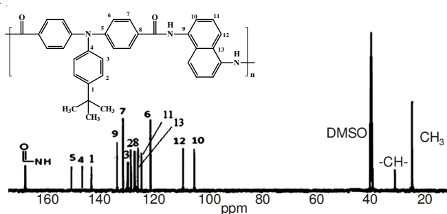
Fig. 11. 13 C NMR of poly(amine-amide) ( pa2 )
