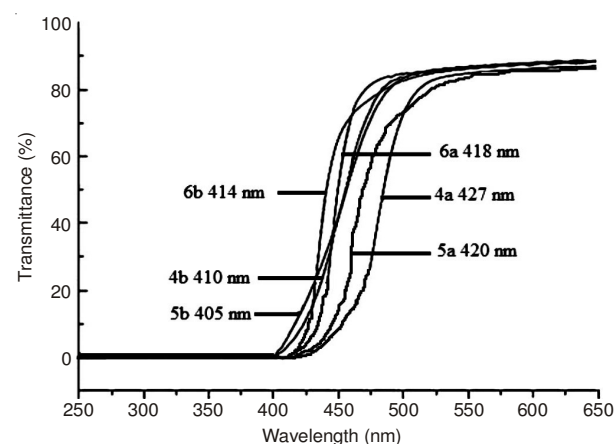
Fig. 16. UV-visible transmittance spectra of poly(amine-amide)s with a concentration (10 -5 M) in NMP
