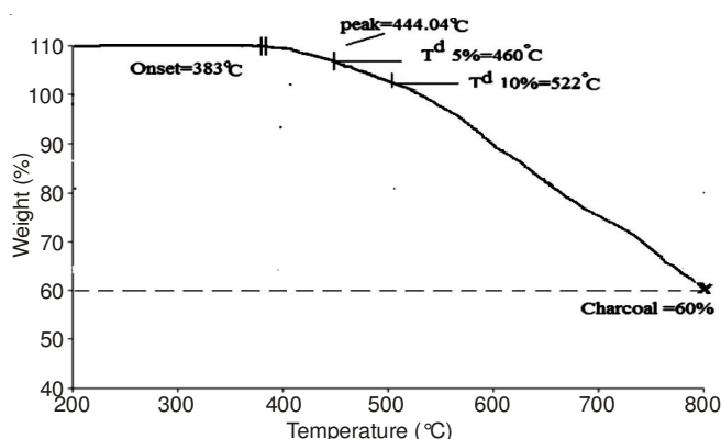
Fig. 13. TGA of Poly(amin-amide) (pa1)
