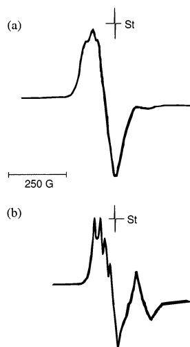
Fig. 7. Experimental X-band ESR spectra of [3e]^+ (a) and [9]^+ (b) in frozen CH_2Cl_2 at liquid nitrogen temperature. St denotes the resonance of LiTCNQ ( g = 2.0025 ).
