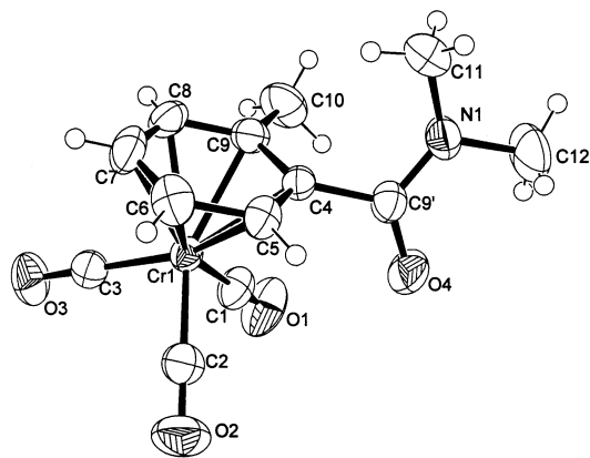
Fig. 2. ORTEP diagram of amide Ila .
