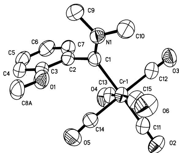
Fig. 3. ORTEP diagram of complex 5c .
