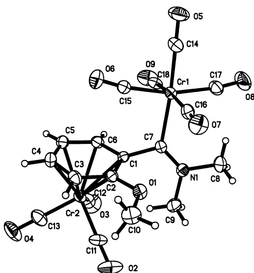
Fig. 4. ORTEP diagram of the complex 6c .
