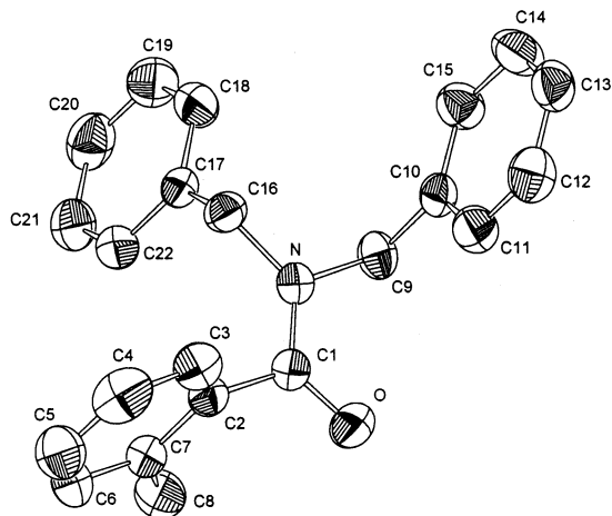
Fig. 1. ORTEP diagram of amide 1b .
