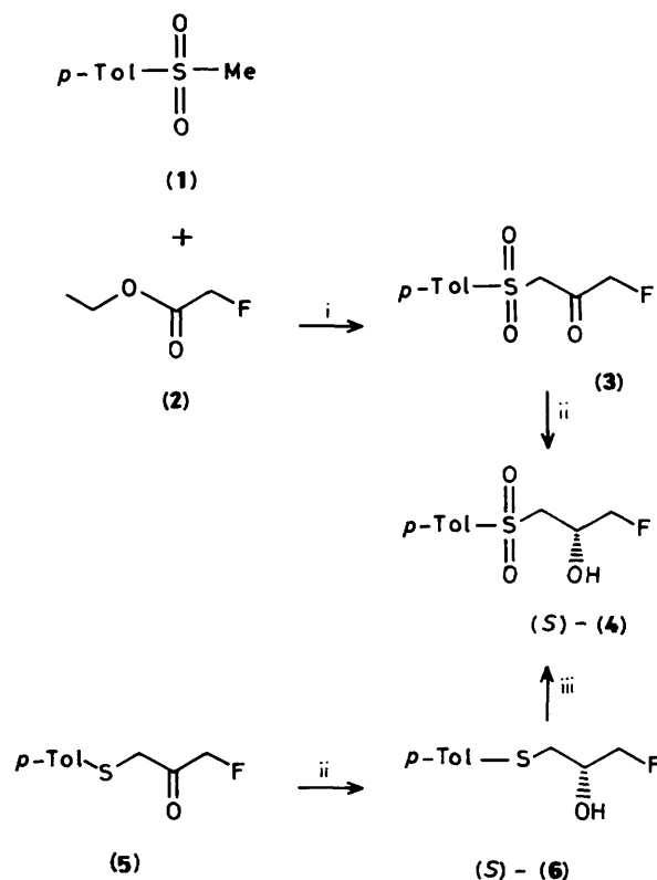
Scheme 1. i, LDA–THF, –78 °C; ii, microbial reduction; iii, KMnO 4 –Bu 4 NBF 4 –CH 2 Cl 2 –water
