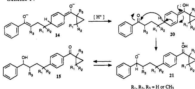
Scheme IV
