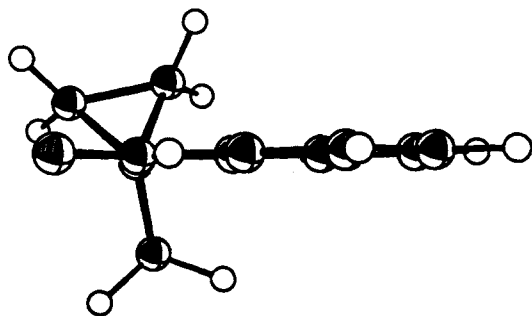
Figure 5. AM1-optimized geometry of (1-benzoyl-1-methylcyclopropyl)ketyl anion ( 9^- ).
