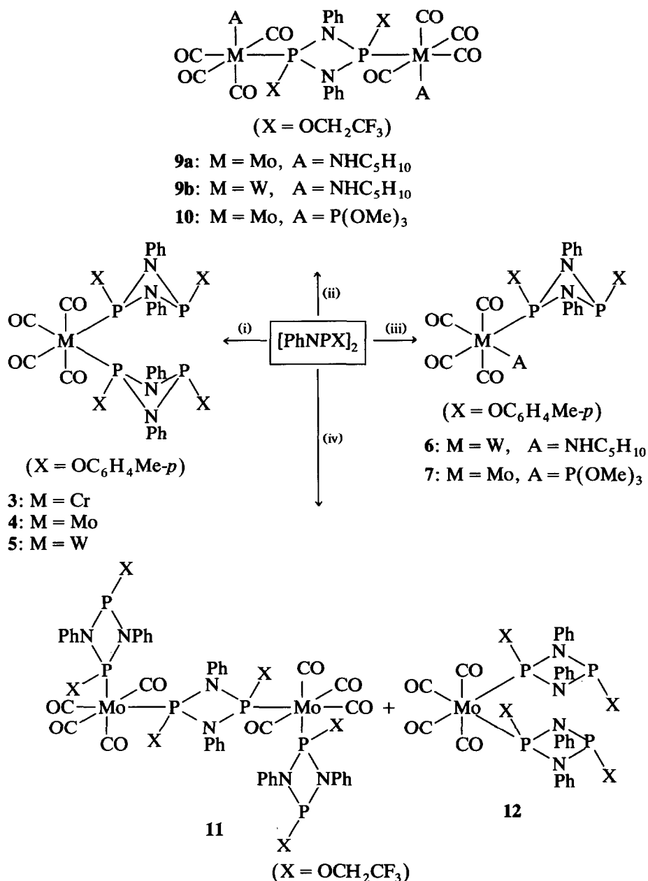
Scheme 1. (i) [\text{M}(\text{CO})_4\text{NBD}] . (ii) [\text{M}(\text{CO})_4(\text{NHC}_5\text{H}_{10})_2] ( \text{M} = \text{Mo}, \text{W} )/ [\text{Mo}(\text{CO})_4\text{P}(\text{OMe})_3] ( \text{NHC}_5\text{H}_{10} ). (iii) [\text{M}(\text{CO})_4(\text{A})(\text{NHC}_5\text{H}_{10})] ( \text{M} = \text{W}, \text{A} = \text{NHC}_5\text{H}_{10} ; \text{M} = \text{Mo}, \text{A} = \text{P}(\text{OMe})_3 ). (iv) [\text{M}(\text{CO})_4\text{NBD}] .
