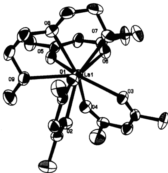
Figure 2. ORTEP drawing of the crystal structure of complex 1. \text{CF}_3 groups have been omitted for clarity. Important bond distances ( \text{\AA} ) are \text{La1-O1} = 2.515(5) , \text{La1-O2} = 2.485(5) , \text{La1-O3} = 2.462(6) , \text{La1-O4} = 2.472(6) , \text{La1-O5} = 2.635(6) , \text{La1-O6} = 2.629(6) , \text{La1-O7} = 2.523(5) , \text{La1-O8} = 2.475(5) , and \text{La1-O9} = 2.642(6) .
