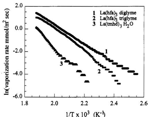
Figure 1. Atmospheric-pressure TGA data of \text{La}(\text{hfa})_3 \cdot \text{diglyme} and \text{La}(\text{hfa})_3 \cdot \text{triglyme} compared to \text{La}(\text{tmhd})_3 \cdot \text{H}_2\text{O} as a function of temperature.
