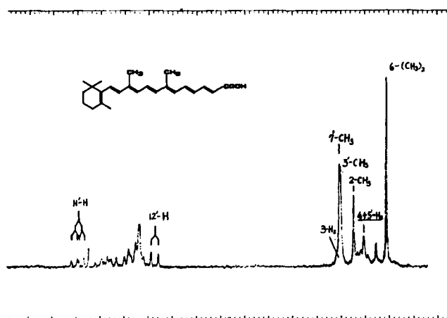
Figure 2—NMR spectrum of \beta - C_{24} acid.
