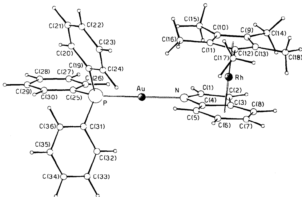
Fig. 1. View of the cationic complex [(C_5Me_5)Rh(\mu\text{-In})AuP(C_6H_5)_3]^{2+} showing the labeling scheme.
