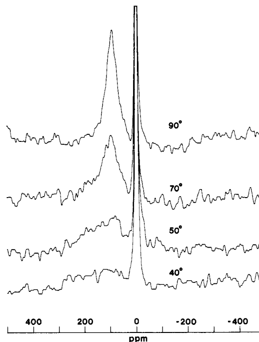
Figure 1. 17 O NMR spectra at 27.1 MHz of [ 17 O]poly A as a function of temperature. Labeled poly A (4 mM in monomeric units) was dissolved in 0.1 M sodium cacodylate buffer containing 0.1 M NaCl and 2 mM EDTA; 17 O-depleted water (0.008% 17 O) was used as the solvent.
