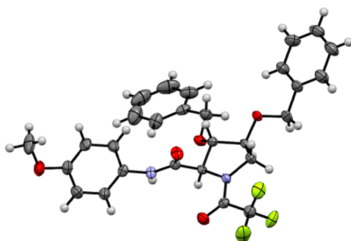
Figure 4. ORTEP plot of 24 with 30% probability ellipsoids.
