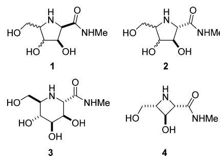
Figure 2. Examples of polyhydroxylated proline amides, pipecolic amide, and azetidine amide derivatives that display high bioactivity against hexosaminidases.
