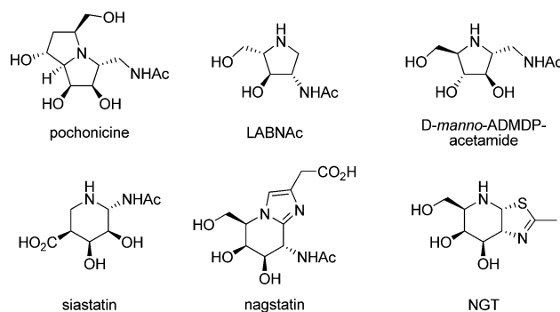
Figure 1. Potent inhibitors of \alpha - and \beta -N-acetylhexosaminidases (HexNAases).
