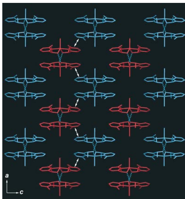
Figure 10. The packing arrangement of \Delta, \Delta - [\text{Co}_2((R)\text{-}\mathbf{3})_2((R)\text{-}\mathbf{3-H})_2\text{Cl}_2] (blue) and \Lambda, \Lambda - [\text{Co}_2((S)\text{-}\mathbf{3})_2((S)\text{-}\mathbf{3-H})_2\text{Cl}_2] (red) in the solid state. The double-headed white arrows indicate \pi - \pi interactions between the pyridyl groups of neighboring helicates, and the dotted blue lines represent hydrogen bonds. Solvent molecules ( \text{CH}_3\text{NO}_2 ) which fill the voids between the helicates are omitted.
