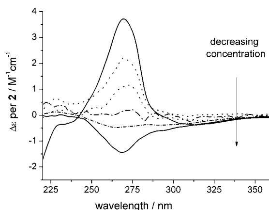
Figure 9. The inversion of the CD spectrum of [\text{Co}_2(\mathbf{2})_2(\mathbf{2}\text{-H})_2\text{Cl}_2] as the concentration is lowered. Spectra measured in \text{CH}_3\text{CN} with effective concentrations of 2 of 22.0, 4.0, 2.0, 1.0, 0.5, 0.2 , and 0.1 \times 10^{-3} \text{ M} .
