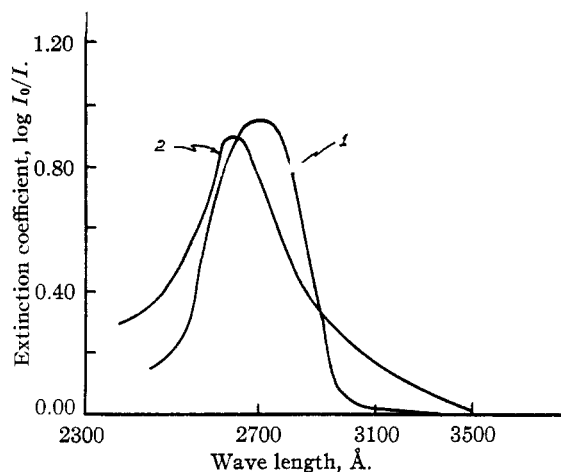
Fig. 2.—Curve 1—Absorption spectra of osajin: maximum at 2730 Å.; solvent, absolute ethyl alcohol; concentration 0.00186 g./100 cc. Cell 0.4 cm. Curve 2—Absorption spectra of iso-osajin: maximum at 2660 Å.; solvent, absolute ethyl alcohol; concentration 0.00142 g./100 cc. Cell, 0.4 cm.
