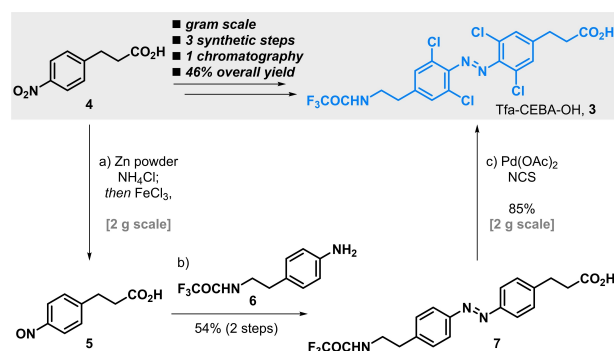
Scheme 1. Synthesis of tetra-ortho-chloro-azobenzene amino acid 3 (Tfa-CEBA-OH). Reaction conditions: a) Zn powder (2.5 equiv), \text{NH}_4\text{Cl} (1.5 equiv), \text{H}_2\text{O} , 2-methoxyethanol, 0^\circ\text{C} to rt, 17 h; then \text{FeCl}_3 (3.0 equiv), EtOH, \text{H}_2\text{O} , 0^\circ\text{C} , 1.5 h. b) 6 (1 equiv), AcOH, rt, 18 h, 54% (2 steps). c) \text{Pd}(\text{OAc})_2 , NCS (6 equiv), AcOH, 140^\circ\text{C} , 19 h, 85%. Tfa = trifluoroacetyl; NCS = N -chlorosuccinimide.
