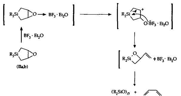
Scheme 10.
