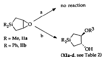
Scheme 8.
