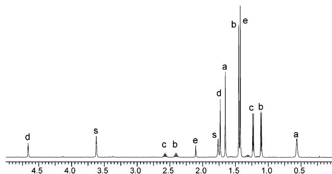
Figure 2. ^1\text{H} NMR monitoring (500 MHz, 20 °C, \text{THF-}d_8 ) of the 1:1 reaction of 4-d 8 with \text{Me}_2\text{CHCO}_2t\text{Bu} [after 3.5 h at 20 °C]. Descriptors a, b, c, d, e, and s refer respectively to 4-d 8 , \text{Me}_2\text{CHCO}_2t\text{Bu} , 5-d 8 , \text{Me}_2\text{C}=\text{CH} , t\text{BuSH} , and residual solvent resonances.
