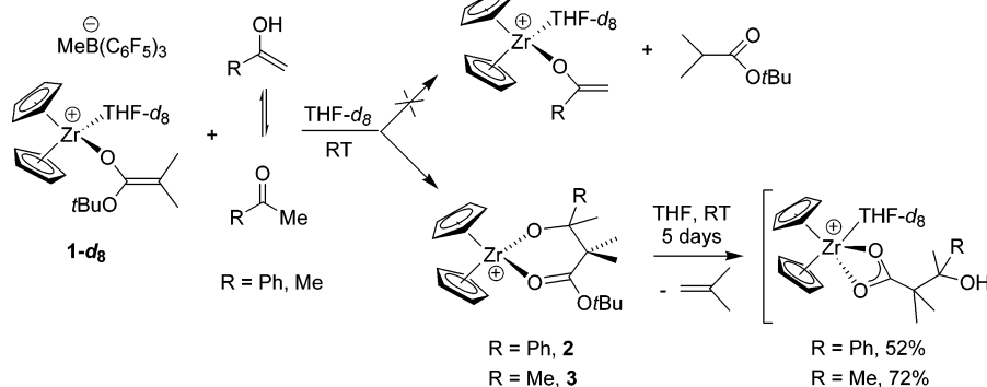
Scheme 3
