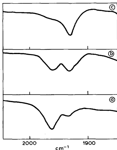
Fig. 1. IR spectra of (\eta^5\text{-C}_5\text{H}_5)\text{Mn}(\text{CO})\text{Ph}_2\text{PCH}_2\text{CH}_2\text{PPh}_2 and \text{CF}_3\text{COOH} solutions in \text{CH}_2\text{Cl}_2 . Complex concentration: 0.01\text{ M} ; acid concentration: 0.1\text{ M} . (a) immediately after preparation; (b) one hour later; (c) after two hours.
