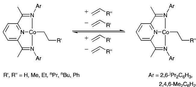
Scheme 5. Reversible Displacement of 1-Alkenes from \text{LCoR} Complexes
