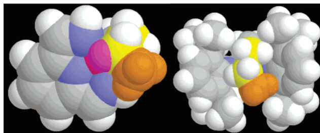
Figure 4. Space-filling representations for (a) 7 with Ar = R = H, showing C–C forming bond (yellow) and methyl (orange) substituent; the alternative endo -facing conformation for the methyl group (replacing the magenta hydrogen) encounters hindrance from the ligand face; and (b) 7 with Ar = 2,6- i Pr 2 C 6 H 3 , R = Me.
