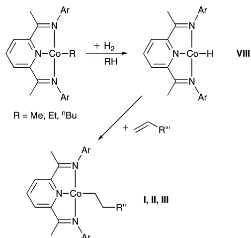
Scheme 4. Preparation of the Cobalt-Hydride Complex VIII and Its Reactivity toward 1-Alkenes
