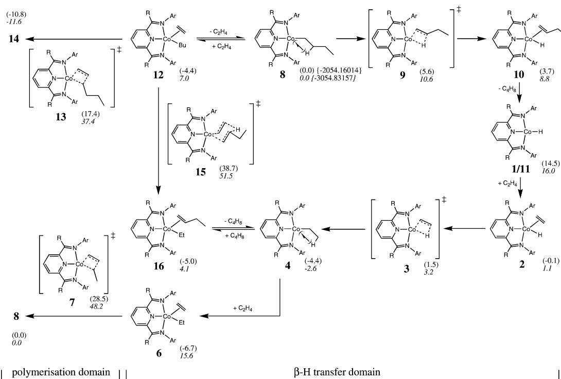
Scheme 7. Scheme for Alkene Exchange a
