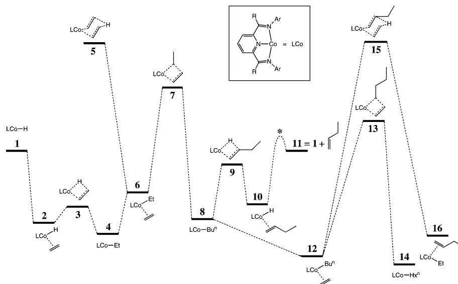
Scheme 6. Schematic for the Free Energy Surface for Stationary Points 1–16 (Ar = R = H) a
