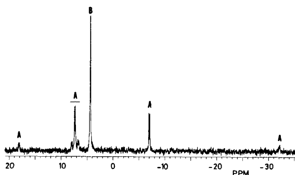
Fig. 2. ^{31}\text{P}\{^1\text{H}\} -NMR spectrum of a dichloromethane solution of A, \text{PtPd}(\text{Ph}_2\text{Ppy})_2\text{Cl}_2 and B, \text{Pd}_2(\text{Ph}_2\text{Ppy})_2\text{Cl}_2 , resulting from the reaction of \text{Pd}(\text{Ph}_2\text{Ppy})_2\text{Cl}_2 with \text{Pt}^\circ(\text{dba})_2 .
