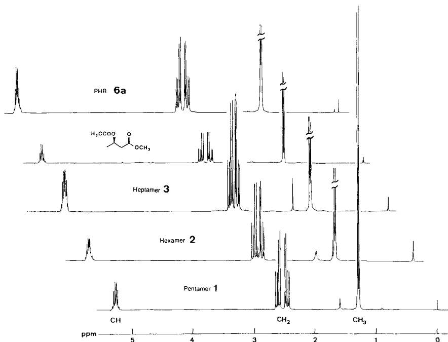
Fig. 4. 300-MHz ^1\text{H} -NMR Spectra ( \text{CDCl}_3 ) of the cyclic oligomers 1 , 2 , and 3 , compared with the acetoxy methyl ester and the polymer PHB. The spectra are recorded at room temperature; concentrations of ca. 10 mg/ml. In the spectrum of the acetoxy ester, the \text{CH}_3\text{CO} and \text{CH}_3\text{O} signals have been deleted. Obviously, there is a striking similarity, almost superimposability of these spectra. This indicates that the average conformations around the \text{CH}_3\text{CH}(\text{OR})\text{CH}_2\text{COOR}' moieties of these species are very similar (for a published ^1\text{H} -NMR spectrum of PHB, see [21b]).
