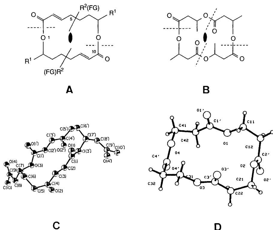
Fig. 1. Comparison of C 2 -symmetrical macrodiolide natural products (A, C) with macrotetrolides from 3-hydroxypropanoic (D) and -butanoic (B). A: General formula representing the natural products pyrenophorine, vermiculine, elaiophylline, and conglobatine [2] [3]; B: 16-membered ring of tetrolide from 3-hydroxybutanoic acid; C 2 -symmetrical structure from four acid moieties of ( R )- or of ( S )-chirality sense; C: X-ray crystal structure of the macrodiolide vermiculine [11]; D: X-ray crystal structure of the tetrolide from 3-hydroxypropanoic acid [12] [13].
