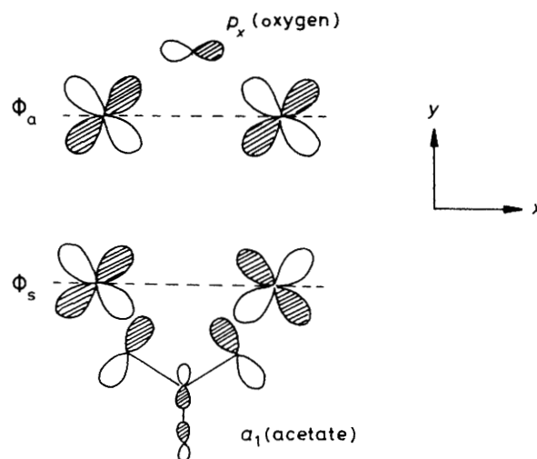
Figure 8. Symmetric ( \varphi_s ) and antisymmetric ( \varphi_a ) combinations of metal d orbitals
