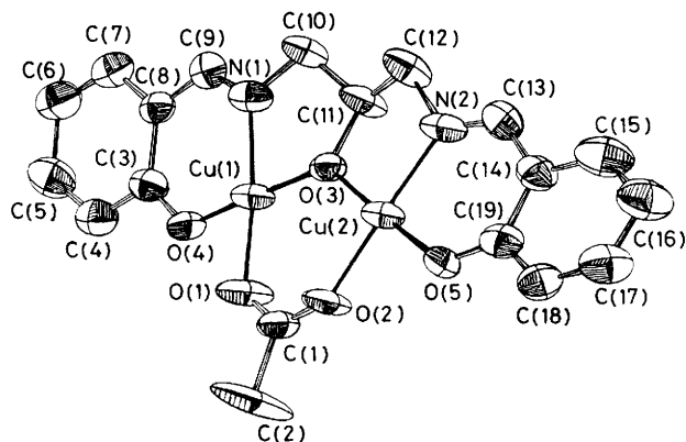
Figure 3. ORTEP drawing of [Cu 2 (L 5 )(O 2 CMe)] (2)
