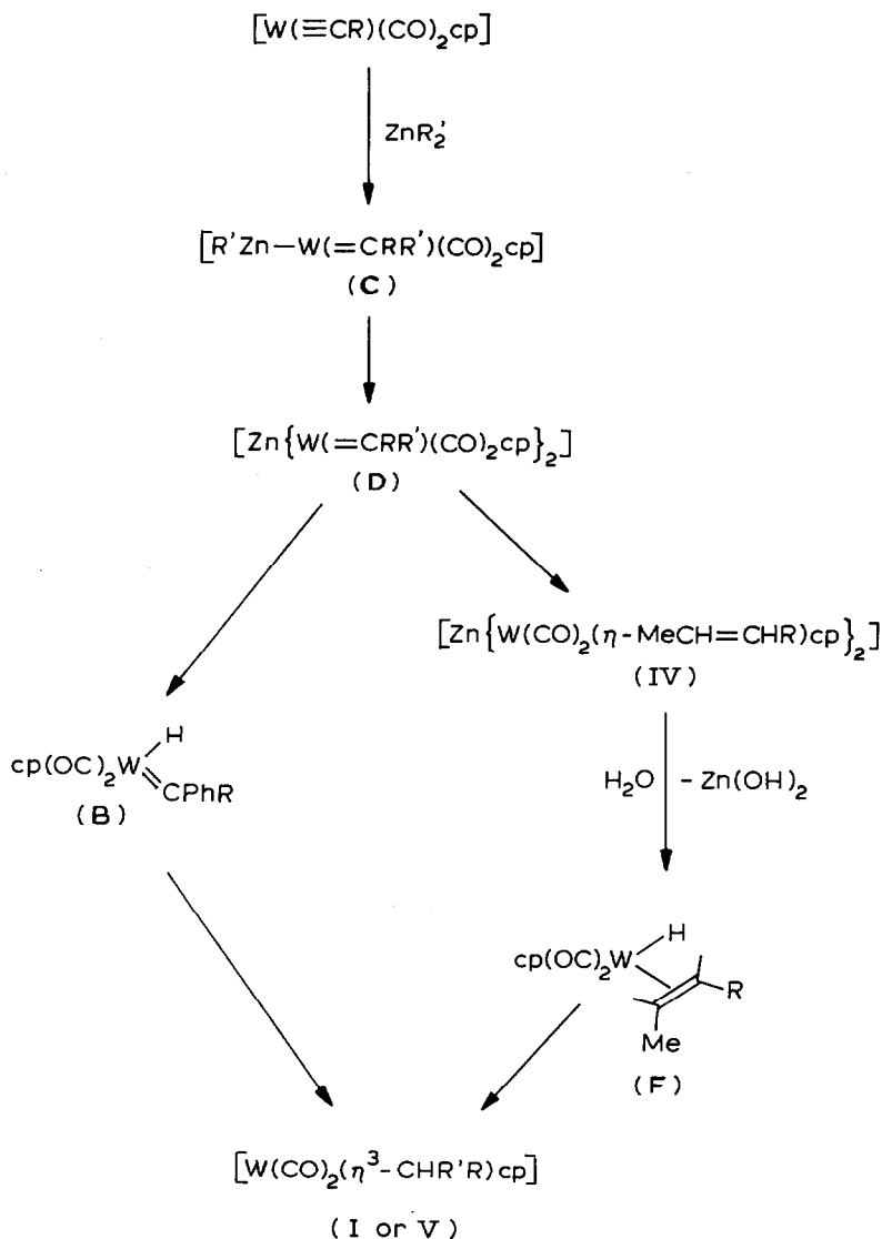
SCHEME 2. cp = \eta\text{-C}_5\text{H}_5 , R = \text{C}_6\text{H}_4\text{Me-4} , R' = \text{Ph} or \text{Et} .
