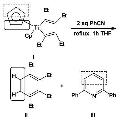
Scheme 1
