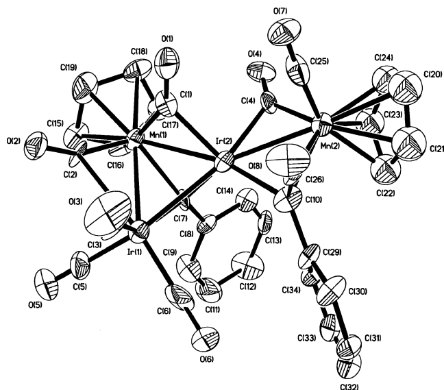
Figure 1. Molecular structure of 6 , showing the atom-numbering scheme with 45% thermal ellipsoids. CH 2 Cl 2 has been omitted for clarity.
