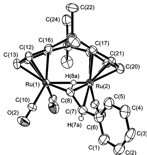
Figure 2. Thermal ellipsoid drawing of the cation in [(\eta^5\text{-C}_5\text{H}_3)_2(\text{SiMe}_2)_2\text{Ru}(\text{CO})_3\{\text{trans-}\mu_2\text{-}\eta^1\text{:}\eta^2\text{-C(H)=C(H)Ph}\}][\text{BF}_4] ( 7 ) with 50% ellipsoid probability and labeling scheme. Hydrogen atoms are omitted for clarity. Selected bond distances (Å) and angles (deg): Ru(1)–Ru(2), 2.878(3); Ru(1)–C(8), 2.105(8); Ru(2)–C(8), 2.118; Ru(2)–C(7), 2.385; C(7)–C(8), 1.389(14); C(6)–C(7), 1.493(14); Ru(1)–Cp(centroid), 1.925; Ru(2)–Cp(centroid), 1.859; \angle\text{C(8)–Ru(1)–Ru(2)} , 47.2(2); \angle\text{C(6)–C(7)–C(8)} , 125.6(9); \angle\text{Ru(1)–C(8)–C(7)} , 129.9(8); \angle\text{Ru(2)–C(8)–C(7)} , 82.91; \angle\text{Ru(1)–C(8)–Ru(2)} , 85.95; \angle\text{Ru(1)–C(8)–C(7)–C(6)} , 8.9; \angle\text{Cp(centroid)–Ru(1)–Ru(2)–Cp(centroid)} , 3.9; \angle\text{Cp–Cp fold angle} , 125.1.
