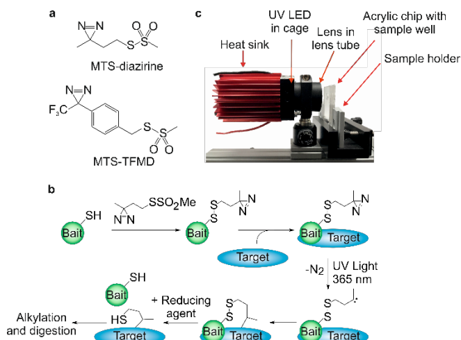
Figure 1. (a) Structures of MTS-diazirine and MTS-TFMD. (b) Crosslinking workflow schematic: A Cys-containing bait protein is conjugated with the reagent (here MTS-diazirine). After adding the target protein, the sample is irradiated with 365 nm UV light, revealing a carbene that reacts with the target. Reductant is added, leaving a sulfhydryl tag on the target at the interaction site. (c) Image of the UV LED lamp and custom-built acrylic chip comprising a 33 \mu L sample well. See also Fig. S4a,b.
