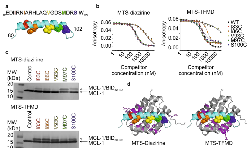
Figure 3. (a) Sequence of WT BID 80-102 . Five Cys variants of BID 80-102 were labelled with MTS-diazirine or MTS-TFMD. Cys-substituted amino acids are shown as coloured spheres in the peptide structure and in the same colour in the sequence above. (b) Inhibitory potency (EC 50 ) of BID 80-102 labelled with MTS-diazirine (left) or MTS-TFMD (right) to MCL-1 measured by fluorescence anisotropy (EC 50 values are shown in Table S1). (c) SDS-PAGE of BID 80-102 labelled with MTS-diazirine (top) or MTS-TFMD (bottom) crosslinked to MCL-1. (d) Residues of MCL-1 (magenta on a grey ribbon) that crosslinked to at least one BID 80-102 peptide labelled with MTS-diazirine (left) or MTS-TFMD (right). BID 80-102 is shown in cyan and residues substituted as Cys are coloured as in (a) (PDB ID: 2KBW [16] ). See also Figs. S6-S8, Tables S2, S3.
