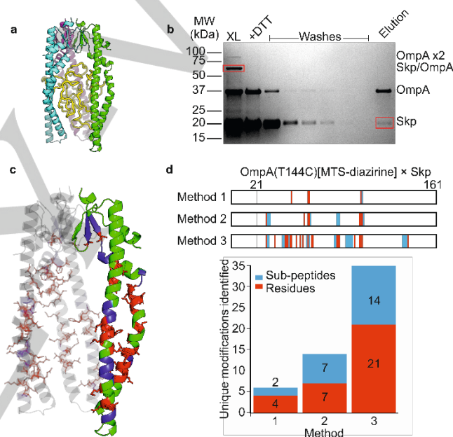
Figure 4. (a) Model of the Skp/OmpA complex. Trimeric Skp (PDB ID: 1U2M [26] ) is shown in cyan, pink and green. Collapsed OmpA (yellow) is shown in the Skp cavity. [25b] (b) Non-reducing SDS-PAGE to show enrichment of crosslinked Skp/OmpA. The crosslinked Skp/OmpA(T144C)[MTS-diazirine] complex (lane 1, XL) was cleaved with DTT. The constituent proteins contain free thiols so can be bound to thiopropyl Sepharose 6B. Unbound material was removed by washing and the captured material eluted by adding DTT. (c) Structure of Skp with crosslinked residues from a pooled dataset of OmpA(T144C)[MTS-diazirine] (Fig. S13, Table S4). One monomer in the Skp trimer is highlighted. In c and d, red represents residue-level information and blue represents crosslinks localised within a 2 or more residue region. (d) Crosslinked residues identified by the enrichment methods shown in Fig. 5 for OmpA(T144C)[MTS-diazirine]. The lower plot shows the total number of unique sites identified by the three enrichment strategies shown in Fig. 5. Representative mass spectra of modified Skp peptides are shown in Figs. S15-S16 and a list of crosslinked peptides is in Tables S4-S5.
