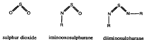
Scheme 1. Imino analogues of sulphur dioxide.
