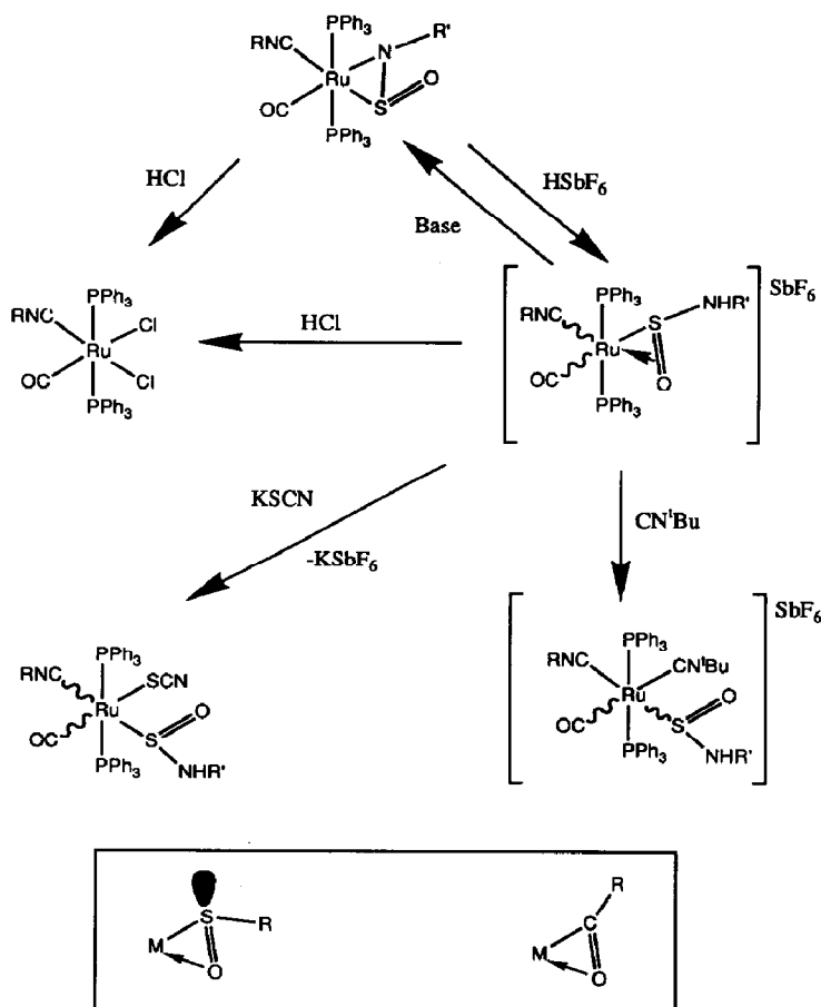
Scheme 2. Protonation of coordinated iminoxosulphuranes ( \text{R} = \text{C}_6\text{H}_3\text{Me}_2\text{-2,6} , \text{R}' = \text{C}_6\text{H}_4\text{Me-4} ).
