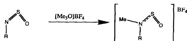
Scheme 3. Alkylation of free iminooxosulphuranes.
