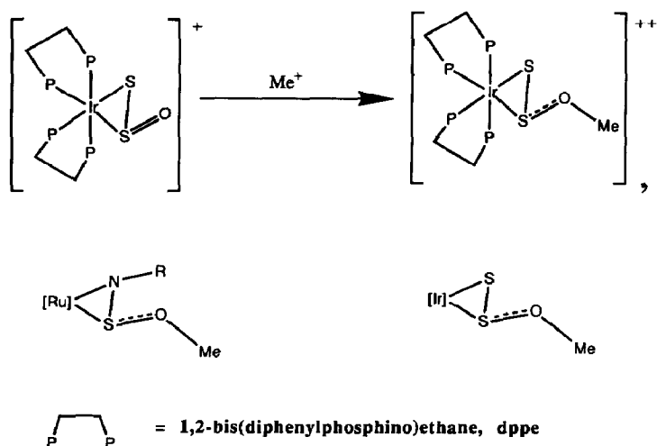
Scheme 5. Alkylation of coordinated disulphur monoxide.
