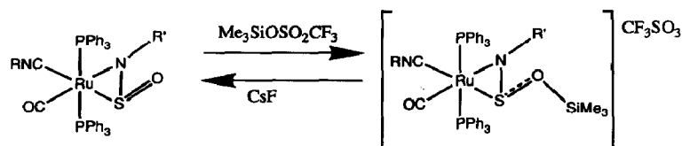
Scheme 6. Silylation of coordinated iminooxosulphuranes \text{R} = \text{C}_6\text{H}_3\text{Me}_2\text{-2,6} , \text{R}' = \text{C}_6\text{H}_4\text{Me-4} ).
