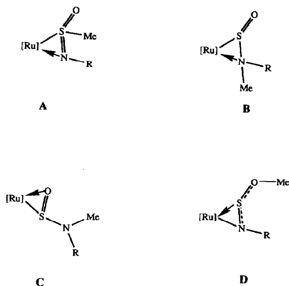
Scheme 4. Isomers for methylation of coordinated iminoxosulphuranes ( [\text{Ru}] = [\text{Ru}(\text{CO})(\text{CNC}_6\text{H}_4\text{Me}_2)(\text{PPh}_3)_2]^+ , \text{R} = \text{C}_6\text{H}_4\text{Me-4} ).
