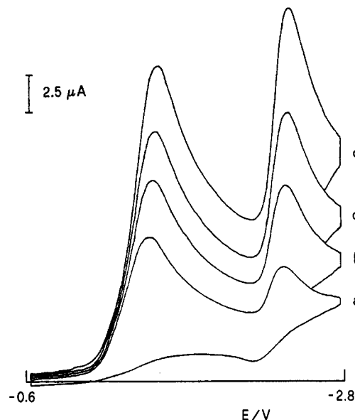
Figure 1. Cyclic voltammeteries for the reduction of 1.2 mM 2-bromo-2-methyl-N-cyclohexylpropanamide in DMF-0.1 M TEAP at different scan rates: Curve a, 1 V s^{-1} ; b, 2 V s^{-1} ; c, 3.16 V s^{-1} ; d, 5 V s^{-1} . T = 25^\circ C .
