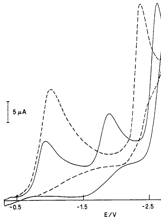
Figure 2. Cyclic voltammograms for the reduction of 3.3 mM 2-bromo-2-methyl- N - p -bromophenylpropanamide in DMF–0.1 M TEAP obtained in the absence (solid curve) or presence of 4 mM acetic acid (dashed curve): T = 25^\circ\text{C} , v = 0.2\text{ V s}^{-1} .
