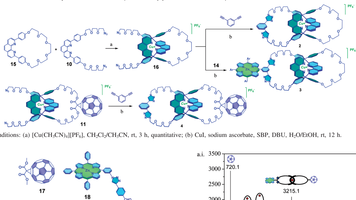
Figure 2. Porphyrin and \text{C}_{60} reference compounds used in the electrochemical and photophysical investigations.
