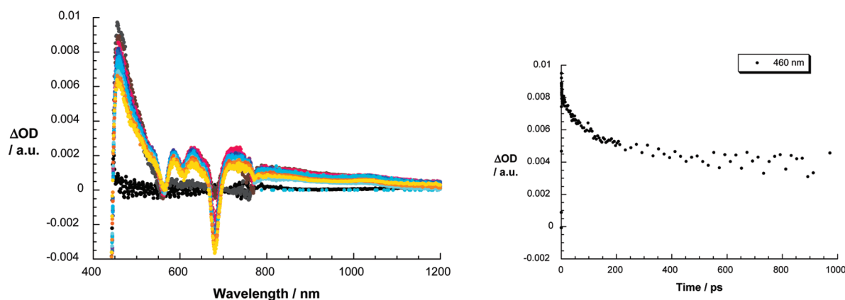
Figure 10. Left: transient absorption spectra (visible and near-infrared) observed upon femtosecond flash photolysis (420 nm, 150 mJ) of ZnP-Cu + -C 60 catenate 1 in benzonitrile with time delays between 0 and 3000 ps at room temperature. Right: time-absorption profiles of the spectra on the left at 460 nm, monitoring the kinetics of energy transfer.
