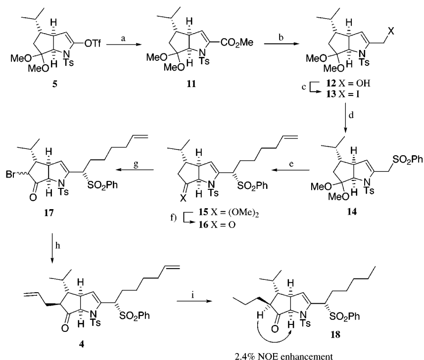
Scheme 3. Attachment of Substituents to Left- and Right-Hand Ring of Bicyclic a
