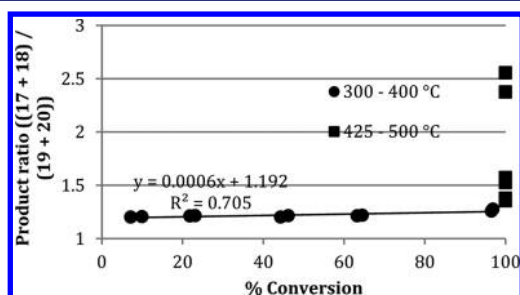
Figure 5. Ratio of [3,5]-sigmatropic rearrangement products (sum of compounds 17 and 18 ) and [3,3]-sigmatropic rearrangement product (sum of compounds 19 and 20 ) from FVP of compound 10 over temperature ranges of 300–400 and 425–500 °C as a function of percent conversion.
