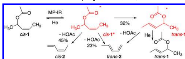
Scheme 2. Initial Product Distribution from MP-IR Irradiation of Z -2-Acetoxy-3-pentene ( cis - 1 ) 4i
