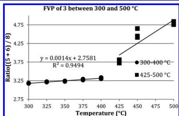
Figure 3. Product ratio of [3,5]-sigmatropic rearrangement products (sum of compounds 5 and 6 ) and [3,3]-sigmatropic rearrangement product (compound 8 ) from FVP of compound 3 over the temperature ranges of 300–400 and 425–500 °C as a function of temperature.
