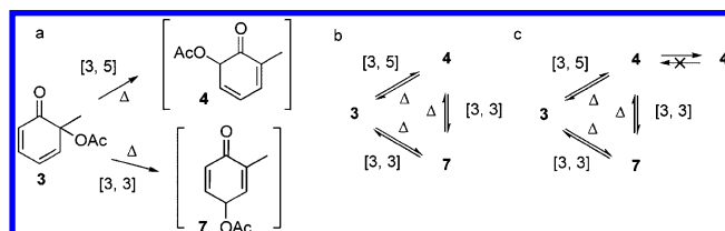
Scheme 7. Possible Mechanistic Pathways for the Formation of Compounds 4 and 7 in the Thermal Rearrangement of Compound 3 : (a) Competing Unimolecular Reactions, (b) Approach to Equilibrium, and (c) Equilibration with Subsequent Irreversible Reaction of Compound 4 to Compound 4'
