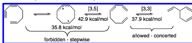
Scheme 1. Calculated (B3LYP/6-31G*) Energies for the Forbidden and, Therefore, Stepwise [3s,5s]-Sigmatropic Rearrangement and the Allowed and, Therefore, Concerted [3s,3s]-Sigmatropic Rearrangement of 1,3,7-Octatriene 2
