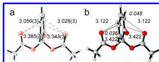
Figure 14. (a) Crystal structure of compound 10 . The thermal ellipsoids are drawn at the 50% probability level. (b) Most stable conformation of compound 10 as calculated at the B3LYP/6-31G(d,p) level of theory. Mulliken charges with hydrogens summed to heavy atoms are shown in italics.
